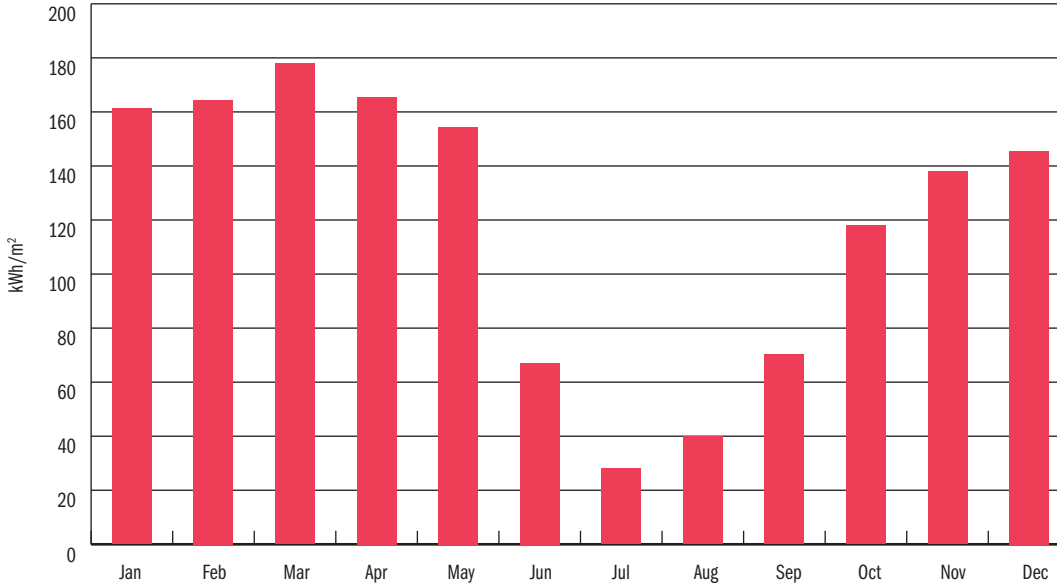
Figure 4.1.3: Monthly average output of photovoltaic power
